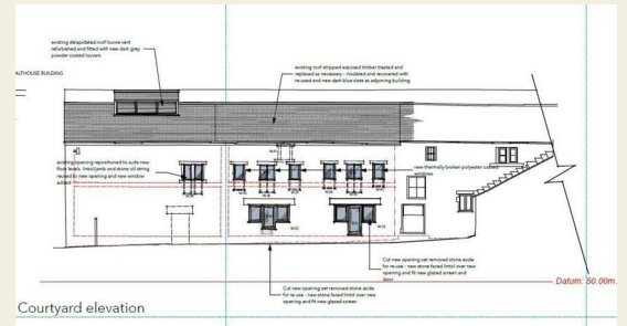
Courtyard elevation
